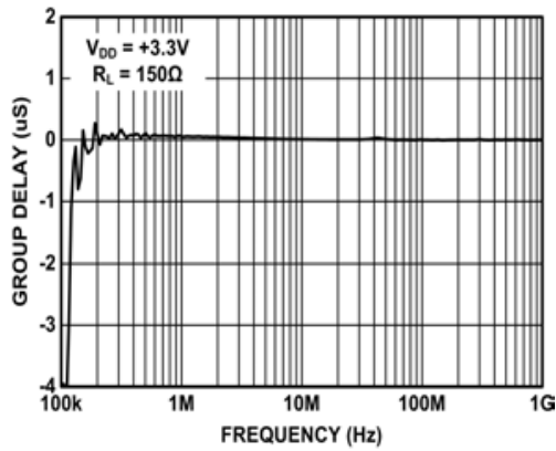
FIGURE 19. GROUP DELAY VERSUS FREQUENCY
