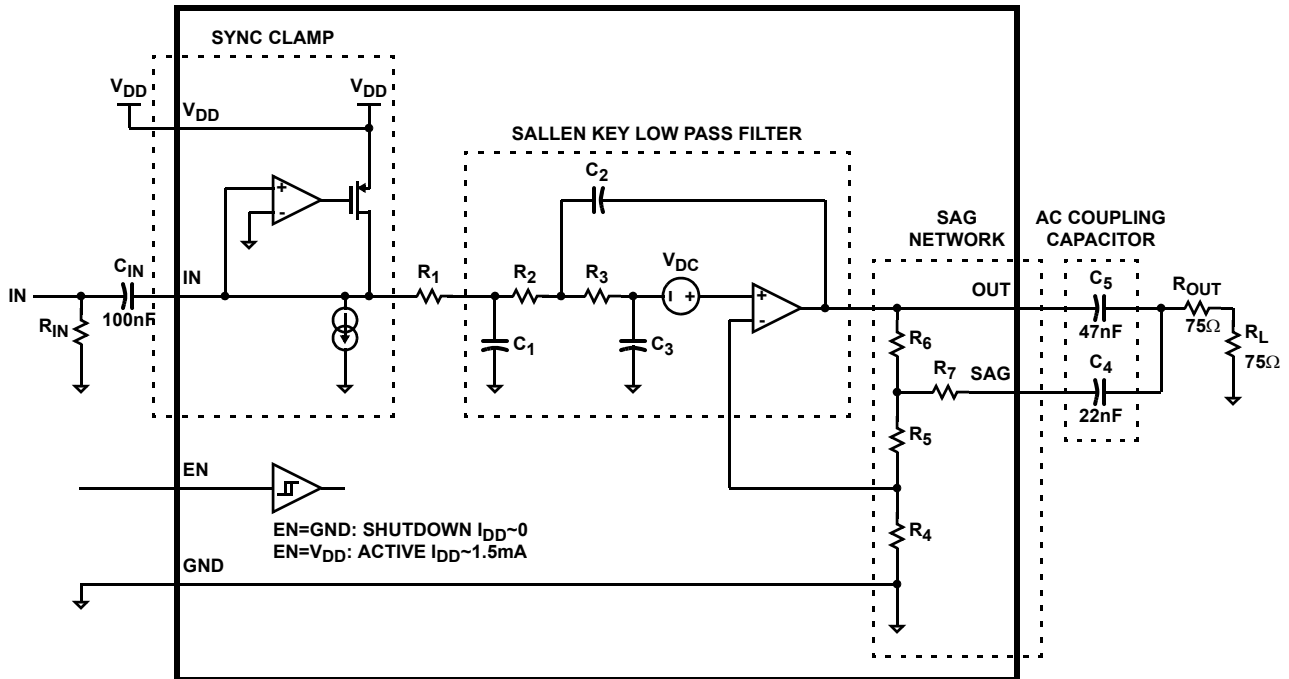
FIGURE 24. BLOCK DIAGRAM
