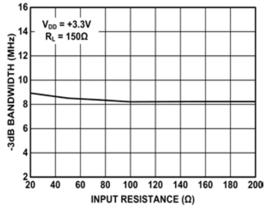
FIGURE 20. -3dB BANDWIDTH VERSUS INPUT RESISTANCE
