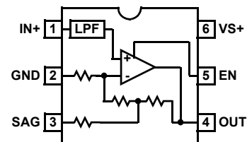
ISL59110 (6-PIN SC-70)* TOP VIEW
