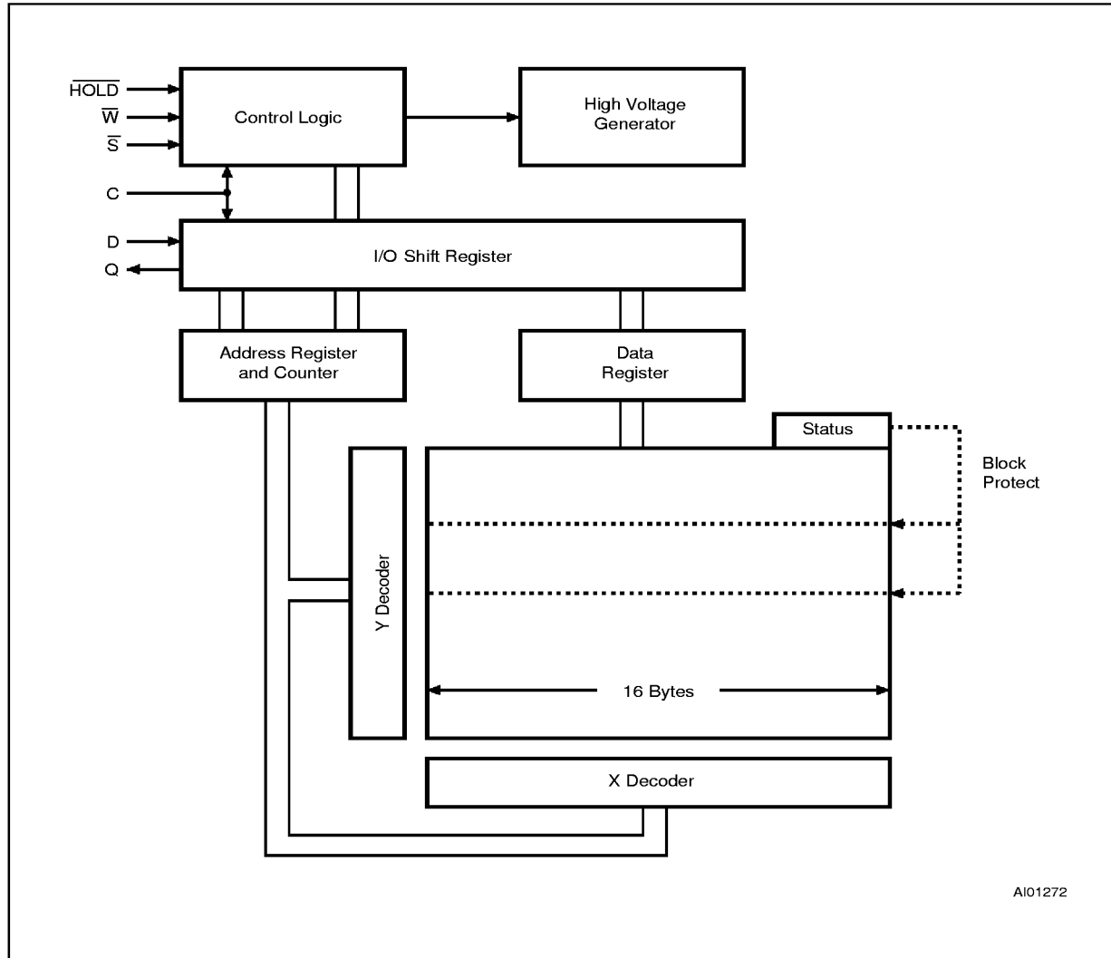
Figure 5. Block Diagram
