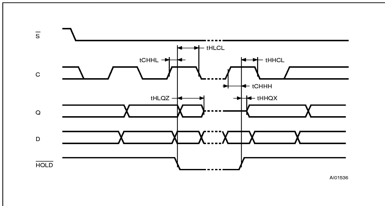
Figure 15. Hold Timing
