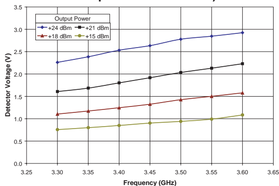
Figure 8: Detector Voltage vs. Frequency ( T_C = +25^\circ\text{C} , V_{CC} = +6.0\text{ V} , V_{BIAS} = +3.0\text{ V} , 54 Mbps OFDM Modulation)
