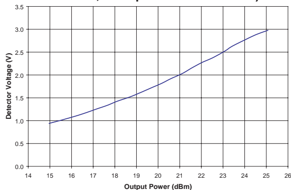
Figure 7: Detector Voltage vs. Output Power ( T_C = +25^\circ\text{C} , V_{CC} = +6.0\text{ V} , V_{BIAS} = +3.0\text{ V} , f = 3.5\text{ GHz} , 54 Mbps OFDM Modulation)
