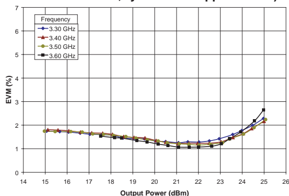
Figure 5: Uncorrected EVM vs. Output Power ( T_C = +25^\circ\text{C} , V_{CC} = +6.0\text{ V} , V_{BIAS} = +3.0\text{ V} , 54 Mbps OFDM Modulation, system EVM Approx. 0.8 %)
