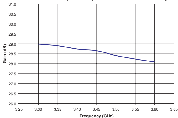
Figure 4: Gain vs. Frequency ( T_C = +25^\circ\text{C} , V_{CC} = +6.0\text{ V} , V_{BIAS} = +3.0\text{ V} , P_{OUT} = +24\text{ dBm} , 54 Mbps OFDM Modulation)
