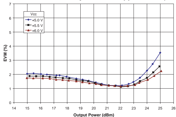
Figure 10: Effects of Supply Voltage ( V_{CC} ) on EVM ( T_C = +25^\circ\text{C} , V_{BIAS} = +3.0\text{ V} , f = 3.5\text{ GHz} , 54 Mbps OFDM Modulation, system EVM Approx. 0.8 %)
