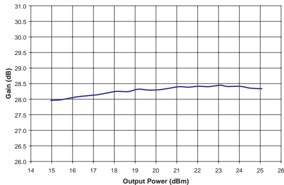
Figure 3: Gain vs. Output Power ( T_C = +25^\circ\text{C} , V_{CC} = +6.0\text{ V} , V_{BIAS} = +3.0\text{ V} , f = 3.5\text{ GHz} , 54 Mbps OFDM Modulation)
