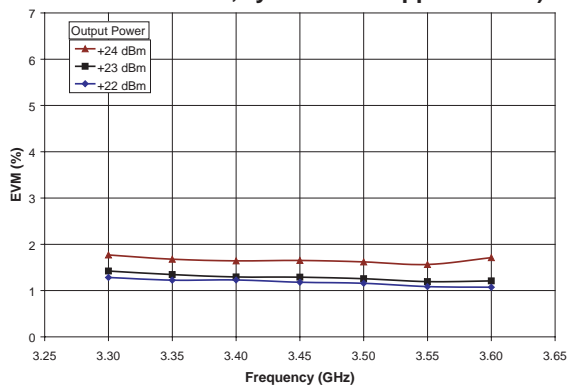
Figure 6: Uncorrected EVM vs. Frequency ( T_C = +25^\circ\text{C} , V_{CC} = +6.0\text{ V} , V_{BIAS} = +3.0\text{ V} , 54 Mbps OFDM Modulation, system EVM Approx. 0.8 %)
