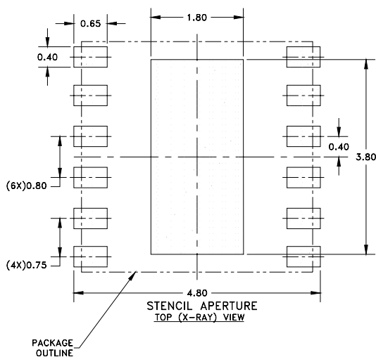
Figure 17: Land Pattern
