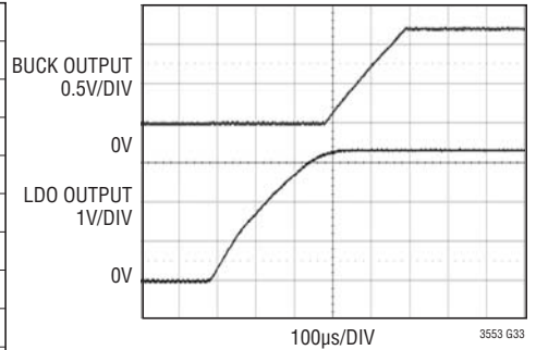
Power-Up Sequencing with SEQ High
