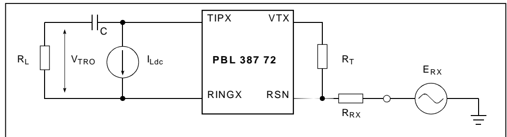
Figure 2. Overload level, V_{\text{TRO}} , two-wire port
