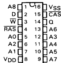
FV PACKAGE (TOP VIEW)
