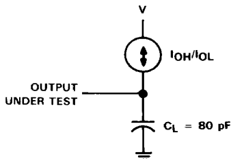
FIGURE 1. EQUIVALENT LOAD CIRCUIT
