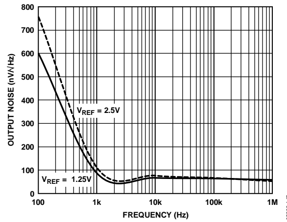
Figure 47. Noise Spectral Density, Internal Reference
