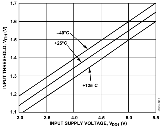
Figure 11. Typical Input Voltage Switching Threshold, Low-to-High Transition
