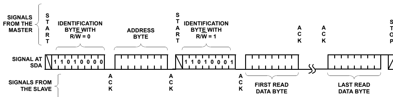
FIGURE 11. READ SEQUENCE
