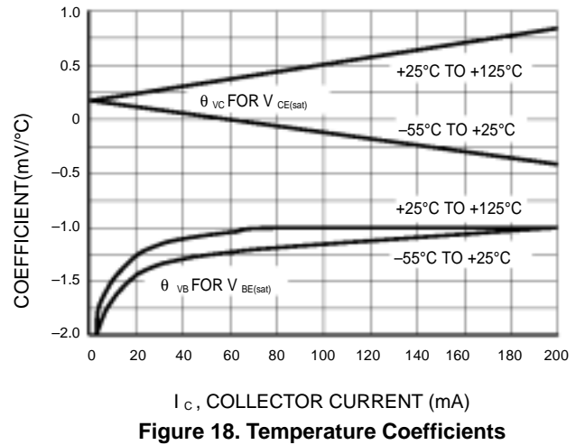
Figure 18. Temperature Coefficients
