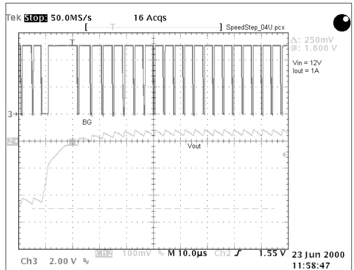
Figure 13 - SpeedStep Transition, 1.35V to 1.60V
