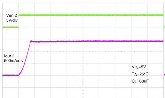
500 \mu s/div Channel 2 Short Circuit Current, Device Enabled Into Short
