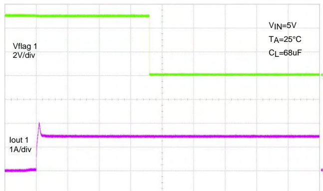
2ms/div Channel 1 2 \Omega Load Connected to Enabled Device
