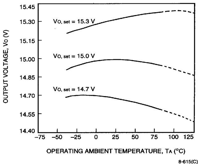
Figure 4. MW005C Typical Output Voltage Variations Over Operating Ambient Temperature Range
