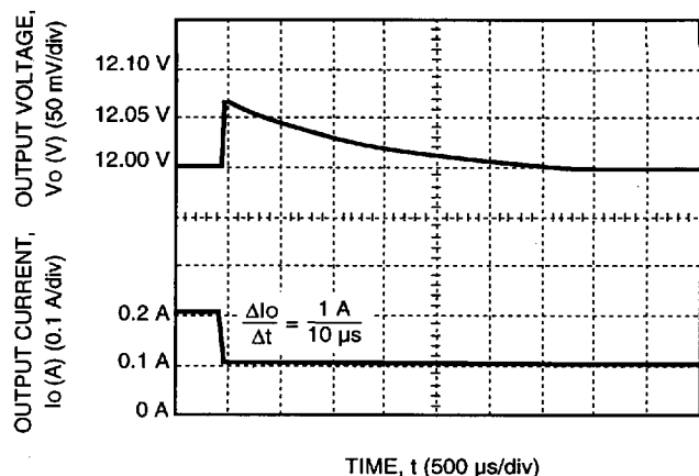
Figure 19. MW005B Typical Output Voltage Waveform for a Step Load Change from 50% to 25% of I_{o,max} with V_i = 48 V and T_A = 25 °C
