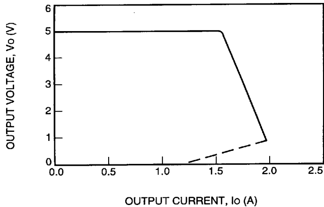
Figure 9. MW005A Typical Output Characteristic with V_i = 48 V and T_A = 25 °C
