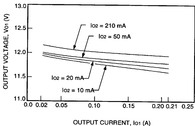
Figure 5. MW005BK Typical V_{O1} vs. I_{O1} Regulation with V_I = 48\text{ V} and T_A = 25^\circ\text{C}
