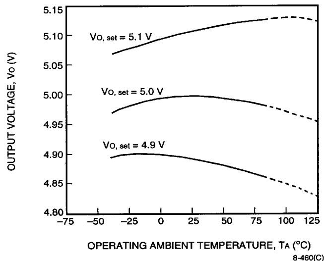
Figure 2. MW005A Typical Output Voltage Variations Over Operating Ambient Temperature Range
