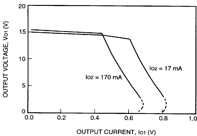
Figure 14. MW005CL Typical Output Characteristics ( V_{O1} vs. I_{O1} ) with V_I = 48 V and T_A = 25 °C
