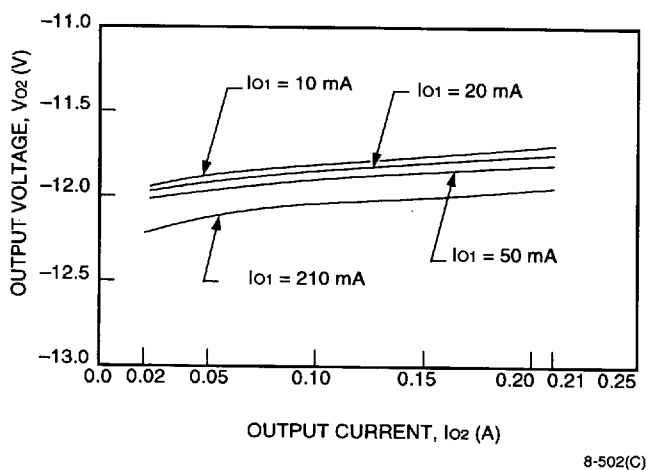
Figure 6. MW005BK Typical V_{O2} vs. I_{O2} Regulation with V_I = 48\text{ V} and T_A = 25^\circ\text{C}
