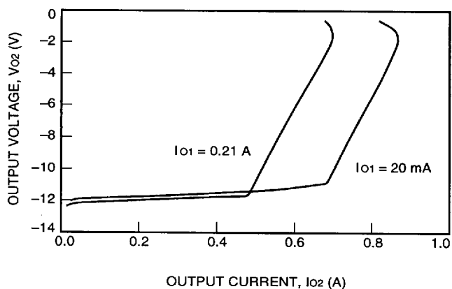
Figure 13. MW005BK Typical Output Characteristics ( V_{O2} vs. I_{O2} ) with V_I = 48 V and T_A = 25 °C
