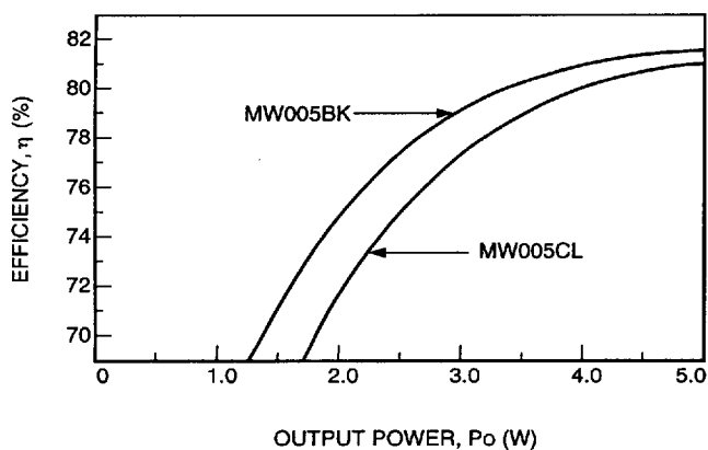
Figure 17. MW005BK, CL Typical Converter Efficiency as a Function of Output Current with V_i = 48 V and T_A = 25 °C
