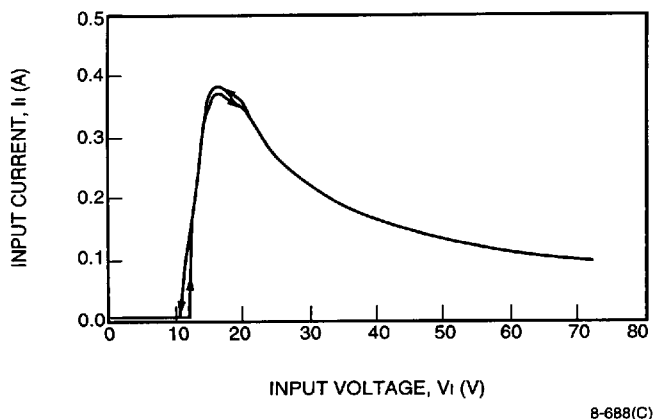
Figure 1. MW005-Series Typical Input Characteristic with I_o = I_{o, max} and T_A = 25^\circ\text{C} (Arrows Indicate Hysteresis)
