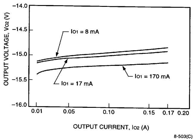
Figure 8. MW005CL Typical V_{O2} vs. I_{O2} Regulation with V_I = 48\text{ V} and T_A = 25^\circ\text{C}
