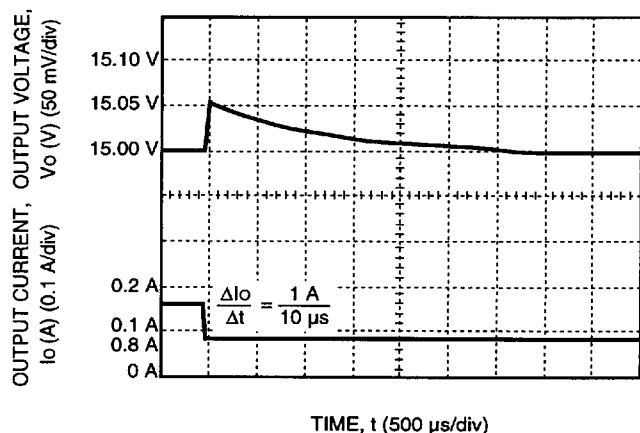
Figure 20. MW005C Typical Output Voltage Waveform for a Step Load Change from 50% to 25% of I_{o,max} with V_i = 48 V and T_A = 25 °C
