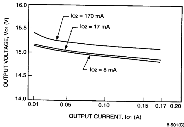
Figure 7. MW005CL Typical V_{O1} vs. I_{O1} Regulation with V_I = 48\text{ V} and T_A = 25^\circ\text{C}
