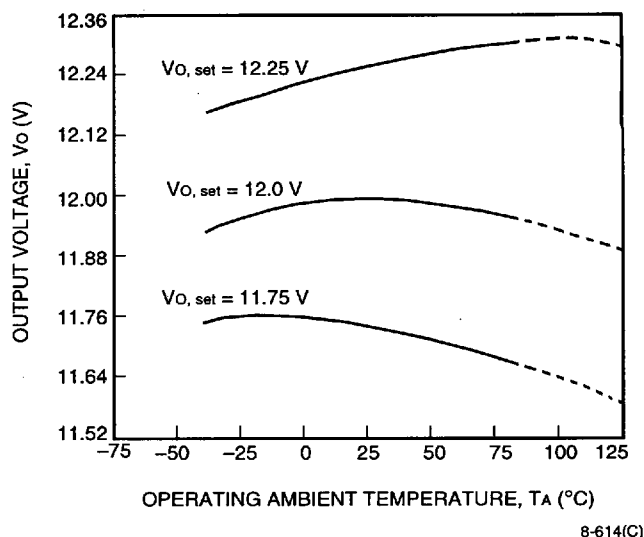
Figure 3. MW005B Typical Output Voltage Variations Over Operating Ambient Temperature Range
