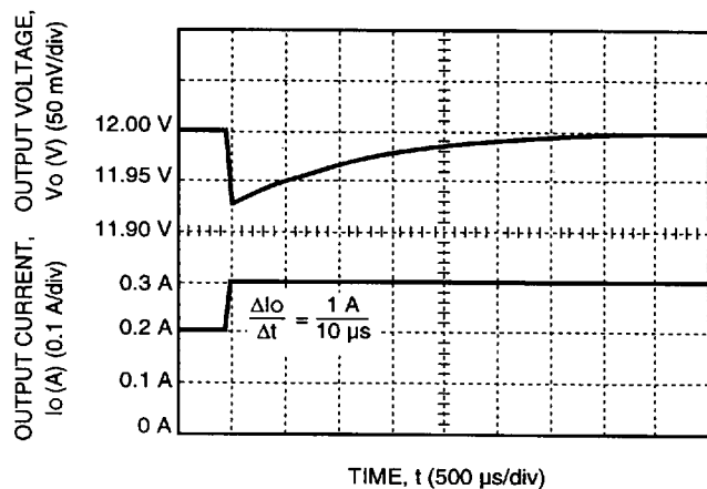
Figure 22. MW005B Typical Output Voltage Waveform for a Step Load Change from 50% to 75% of I_{o,max} with V_i = 48 V and T_A = 25 °C
