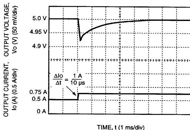
Figure 21. MW005A Typical Output Voltage Waveform for a Step Load Change from 50% to 75% of I_{o,max} with V_i = 48 V and T_A = 25 °C
