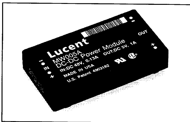
The MW005-Series Power Modules are encapsulated in nonconductive cases measuring 50.8 mm long, 27.9 mm wide, and 11.7 mm high (2.00 in. x 1.10 in. x 0.46 in.).
