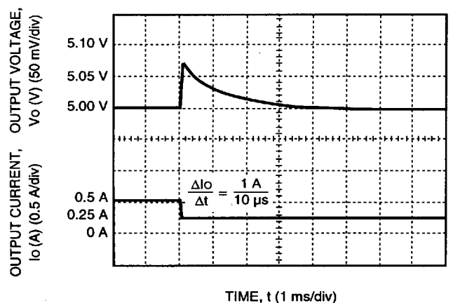
Figure 18. MW005A Typical Output Voltage Waveform for a Step Load Change from 50% to 25% of I_{o,max} with V_i = 48 V and T_A = 25 °C
