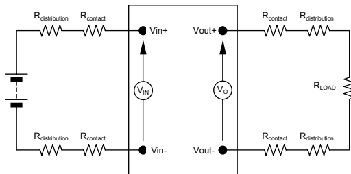
Figure 14. Output Ripple and Noise Test Setup.
