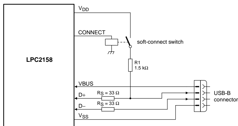
Fig 11. LPC2158 USB interface using the CONNECT function on pin 17
