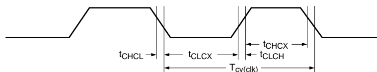
Fig 9. External clock timing (with an amplitude of at least V_{i(RMS)} = 200 mV)
