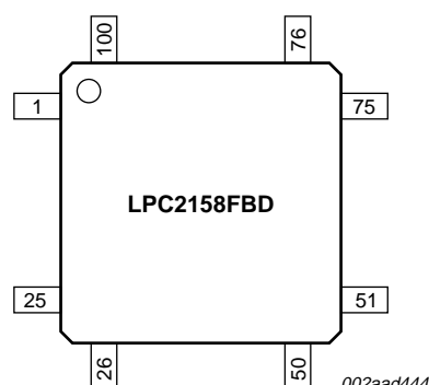
Fig 5. Pin configuration for LPC2158
