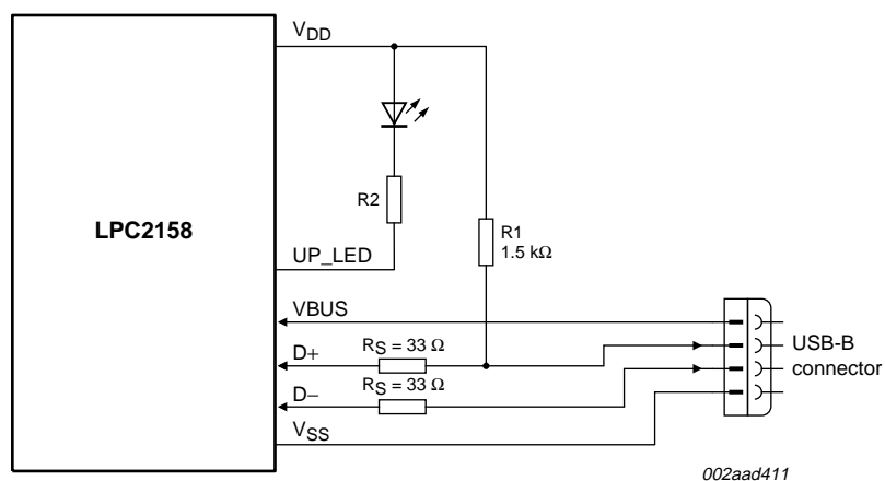
Fig 12. LPC2158 USB interface using the UP_LED function on pin 17
