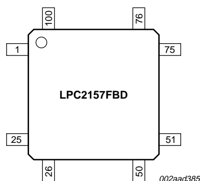
Fig 4. Pin configuration for LPC2157
