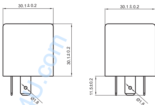
Outline Dimensions
