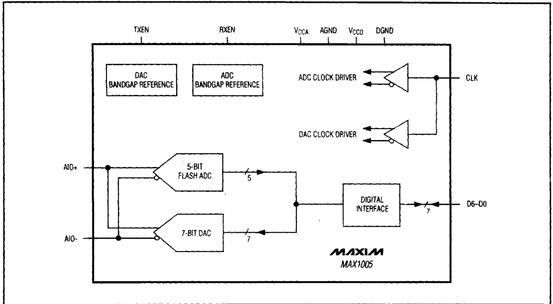
Functional Diagram
