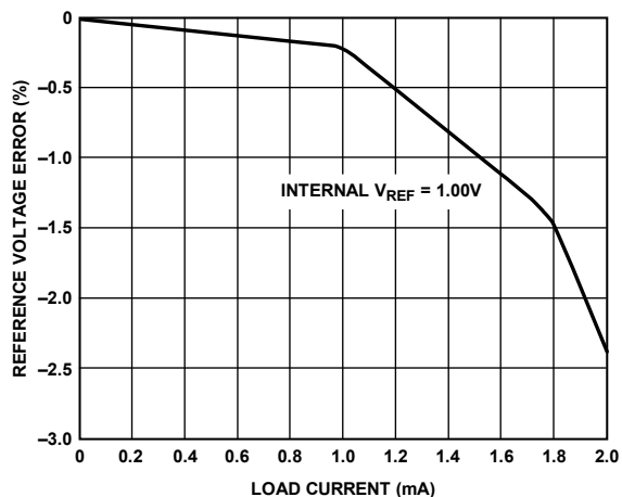
Figure 50. VREF Accuracy vs. Load Current
