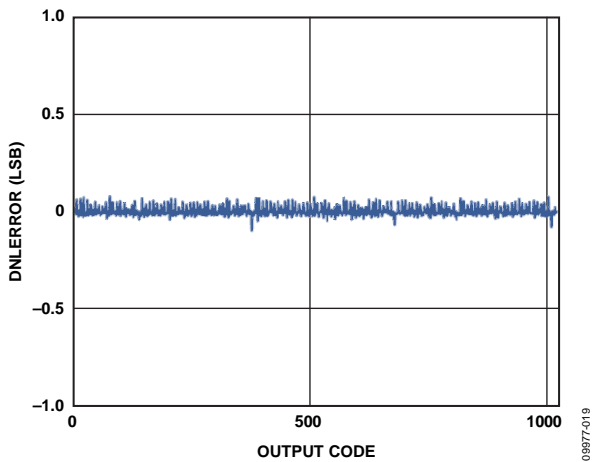
Figure 30. DNL Error with f_{IN} = 9.7 MHz
