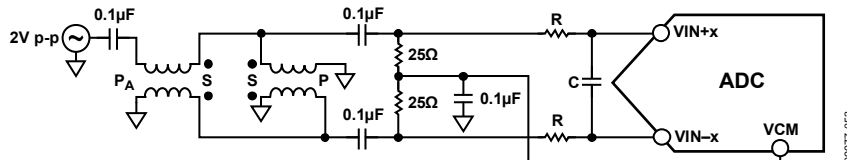
Figure 46. Differential Double Balun Input Configuration
