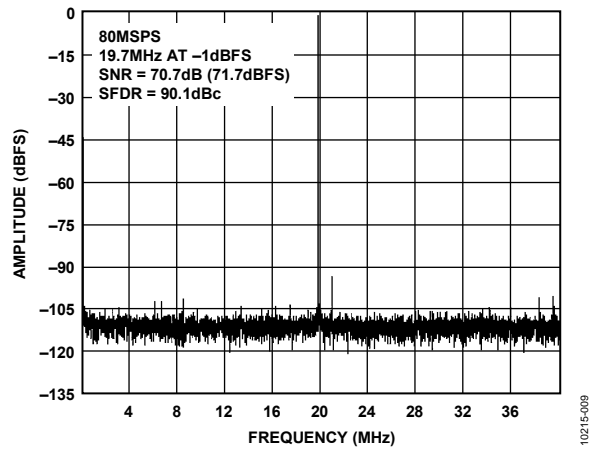
Figure 9. Single-Tone 16k FFT with f_{IN} = 19.7 MHz, f_{SAMPLE} = 80 MSPS
