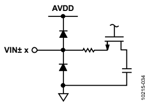
Figure 35. Equivalent Analog Input Circuit
