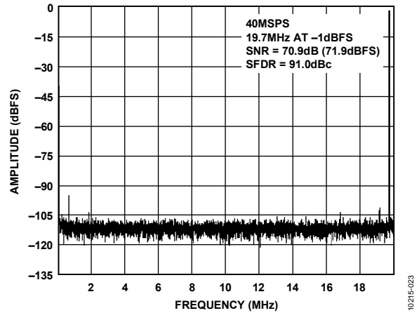
Figure 24. Single-Tone 16k FFT with f_{IN} = 19.7 MHz, f_{SAMPLE} = 40 MSPS
