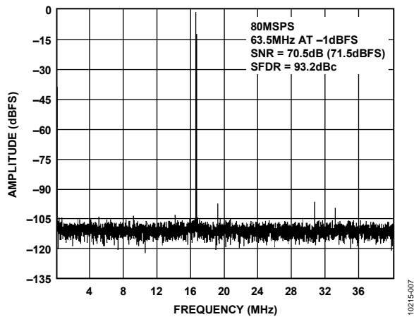
Figure 7. Single-Tone 16k FFT with f_{IN} = 63.5 MHz, f_{SAMPLE} = 80 MSPS
