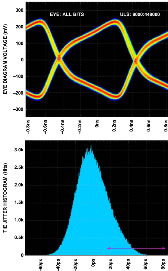
Figure 59. Data Eye for LVDS Outputs in ANSI-644 Mode with Trace Lengths of Less Than 24 Inches on Standard FR-4, External 100 Ω Far-End Termination Only
