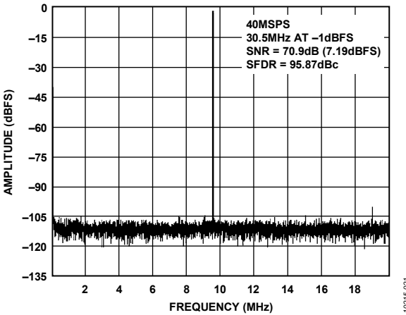
Figure 22. Single-Tone 16k FFT with f_{IN} = 30.5 MHz, f_{SAMPLE} = 40 MSPS
