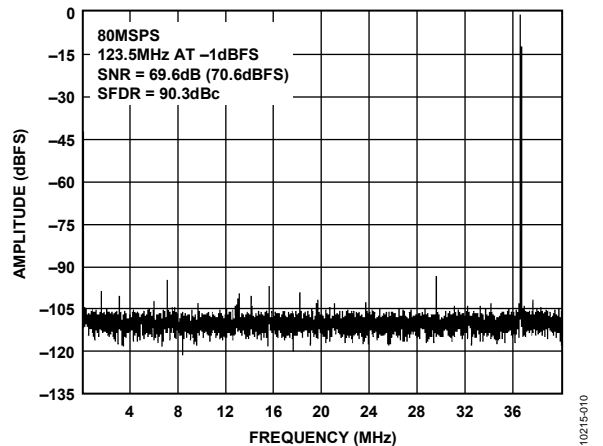
Figure 11. Single-Tone 16k FFT with f_{IN} = 123.5 MHz, f_{SAMPLE} = 80 MSPS
