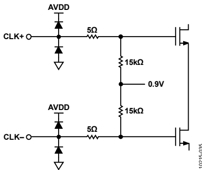
Figure 36. Equivalent Clock Input Circuit
