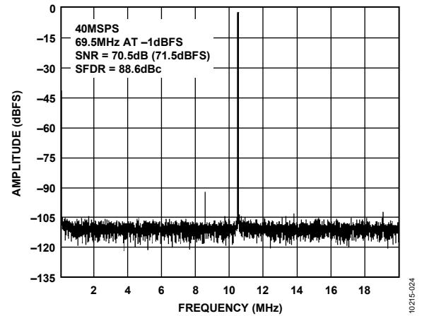
Figure 25. Single-Tone 16k FFT with f_{IN} = 69.5 MHz, f_{SAMPLE} = 40 MSPS
