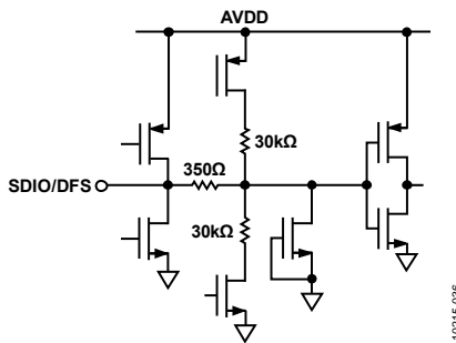
Figure 37. Equivalent SDIO/DFS Input Circuit
