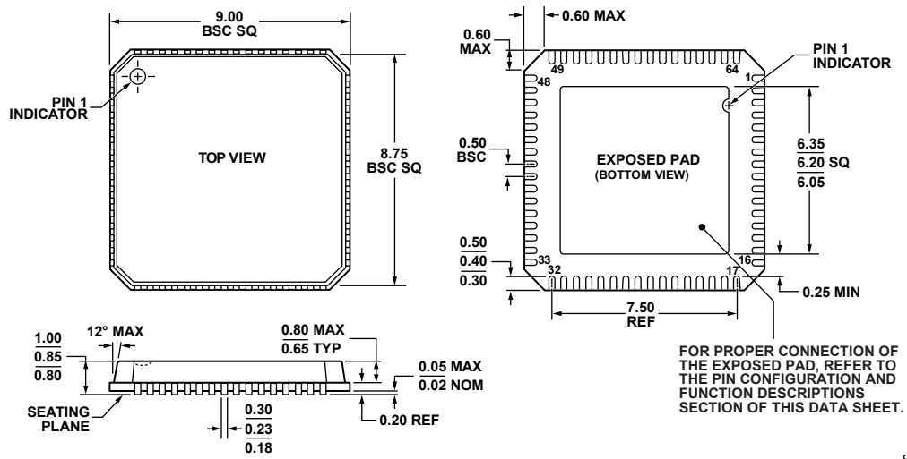
Figure 62. 64-Lead Lead Frame Chip Scale Package [LFCSP_VQ] 9 mm × 9 mm Body, Very Thin Quad (CP-64-4) Dimensions shown in millimeters
