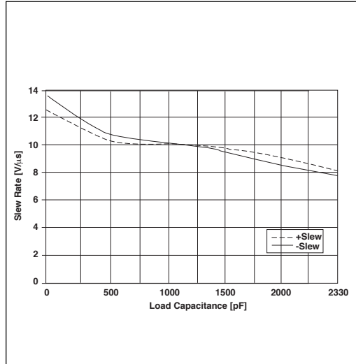
Figure 2. Slew Rate VS. Load Capacitance for the SP3222H and the SP3232H
