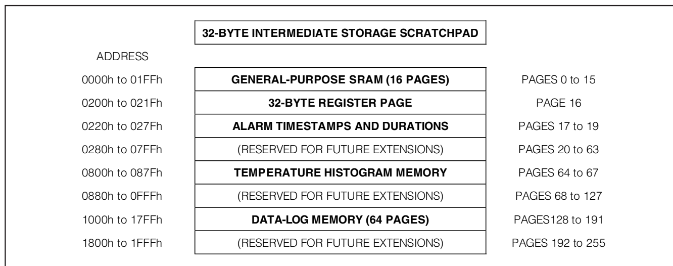
Figure 5. Memory Map
