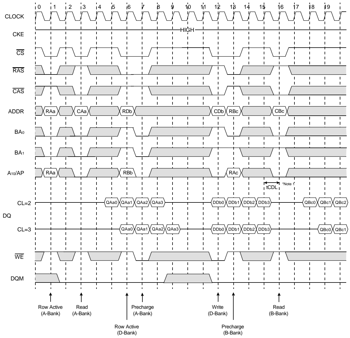
Read & Write Cycle at Different Bank @Burst Length=4
