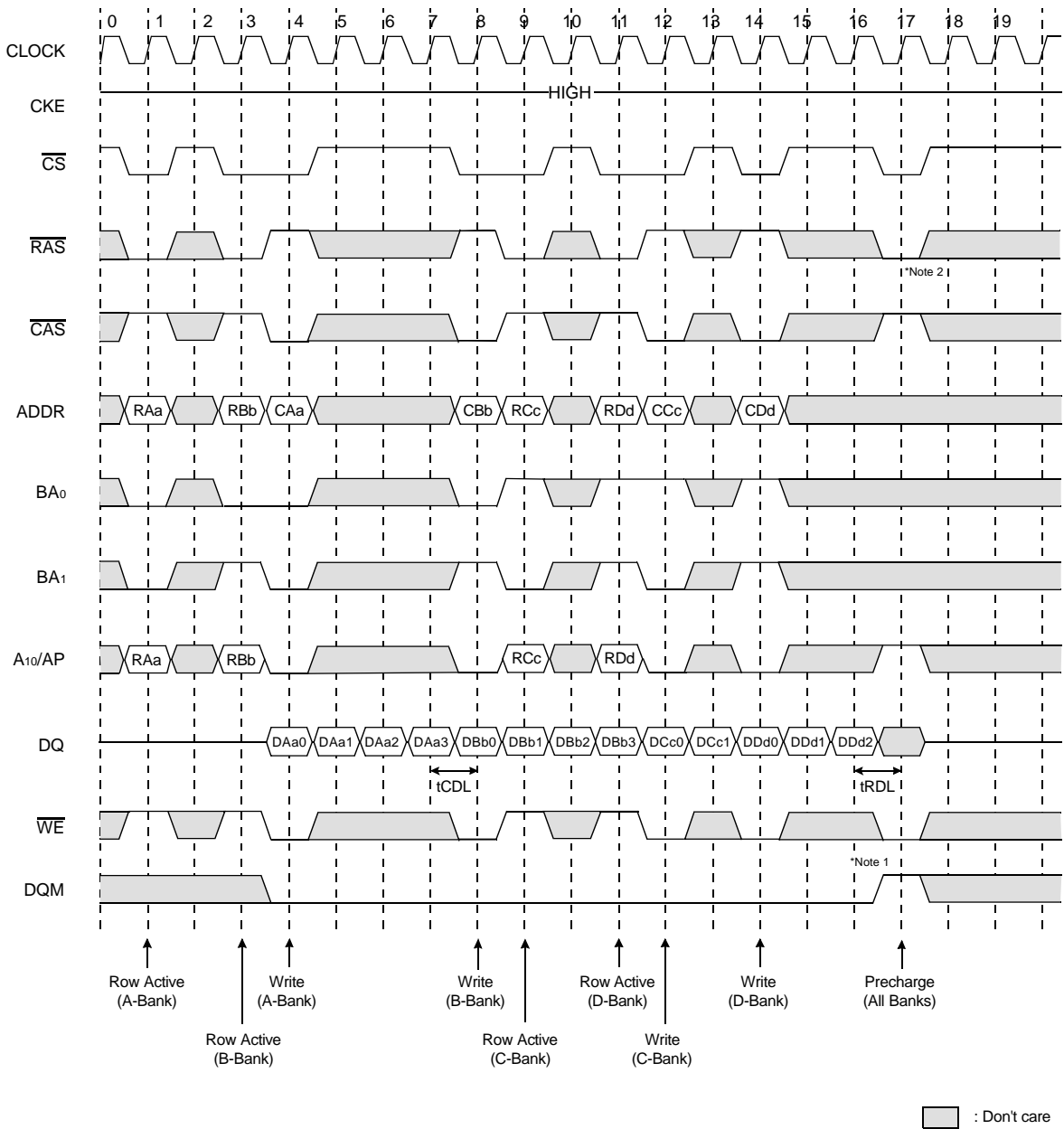
Page Write Cycle at Different Bank @Burst Length=4
