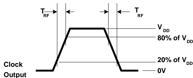
Figure 4. Rise Time = T RF Fall Time = T RF
