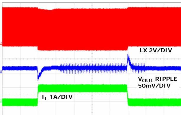
FIGURE 17. LOAD TRANSIENT (PWM), 200\mu\text{s}/\text{DIV}
