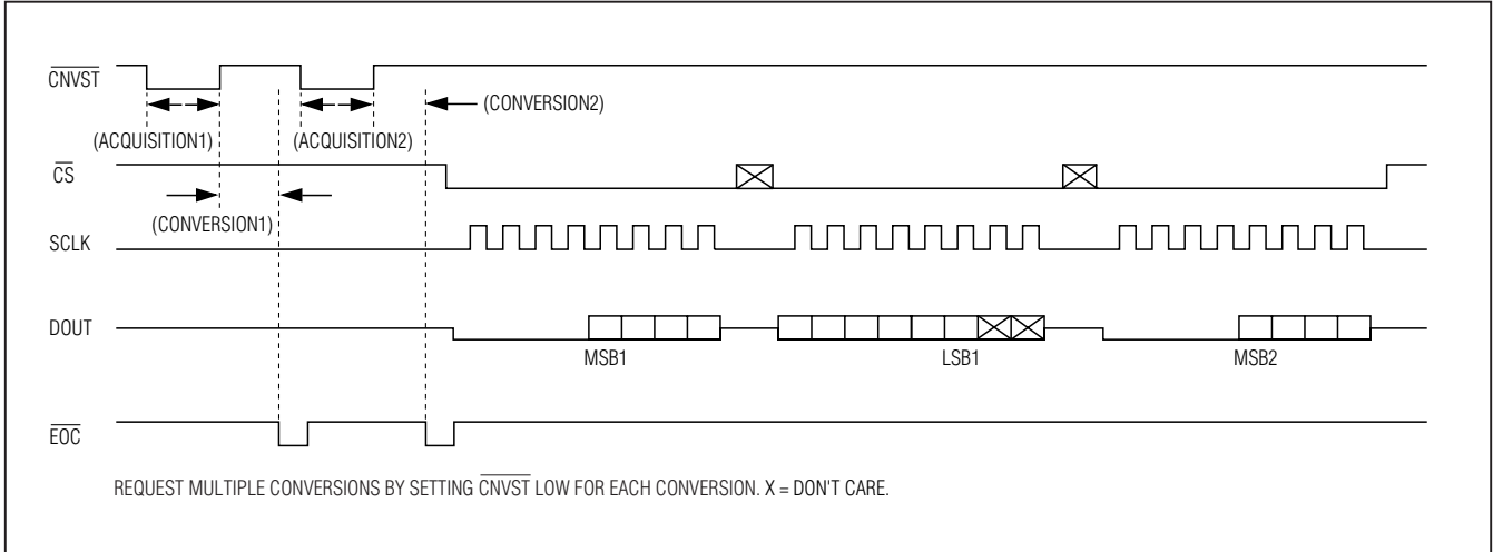
Figure 5. Clock Mode 01
