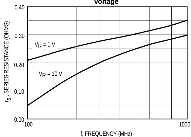
Figure 4. Series Resistance versus Frequency
