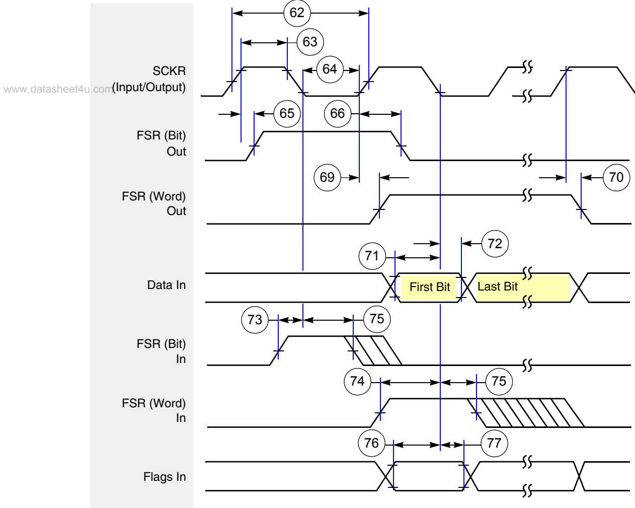
Figure 21. ESAI Receiver Timing Diagram
