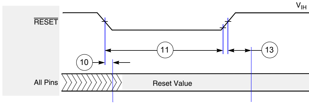
Figure 11. Reset Timing Diagram
