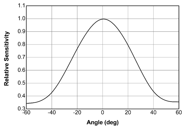
Fig.5 Relative Sensitivity vs. Angle
