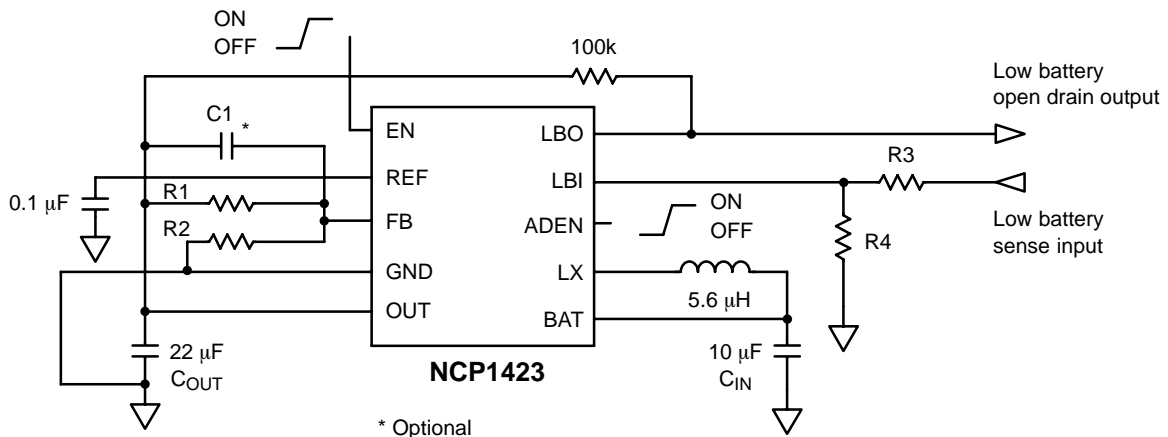
* Optional Figure 1. Typical Operation Circuit
