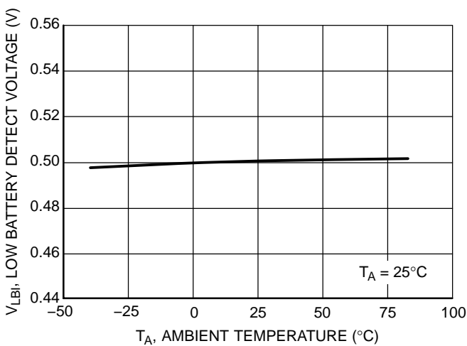
Figure 7. Low Battery Detect Voltage vs. Temperature
