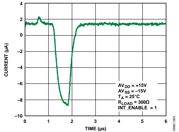
Figure 46. Current vs. Time on Output Enable
