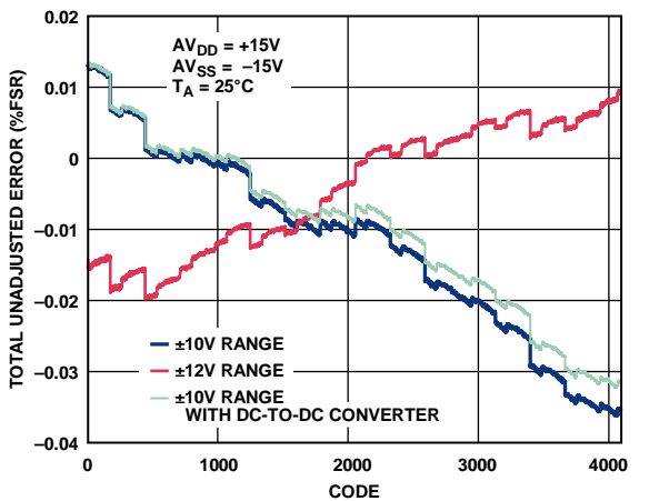
Figure 10. Total Unadjusted Error vs. DAC Code
