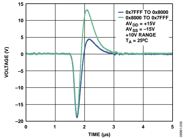
Figure 25. Digital-to-Analog Glitch
