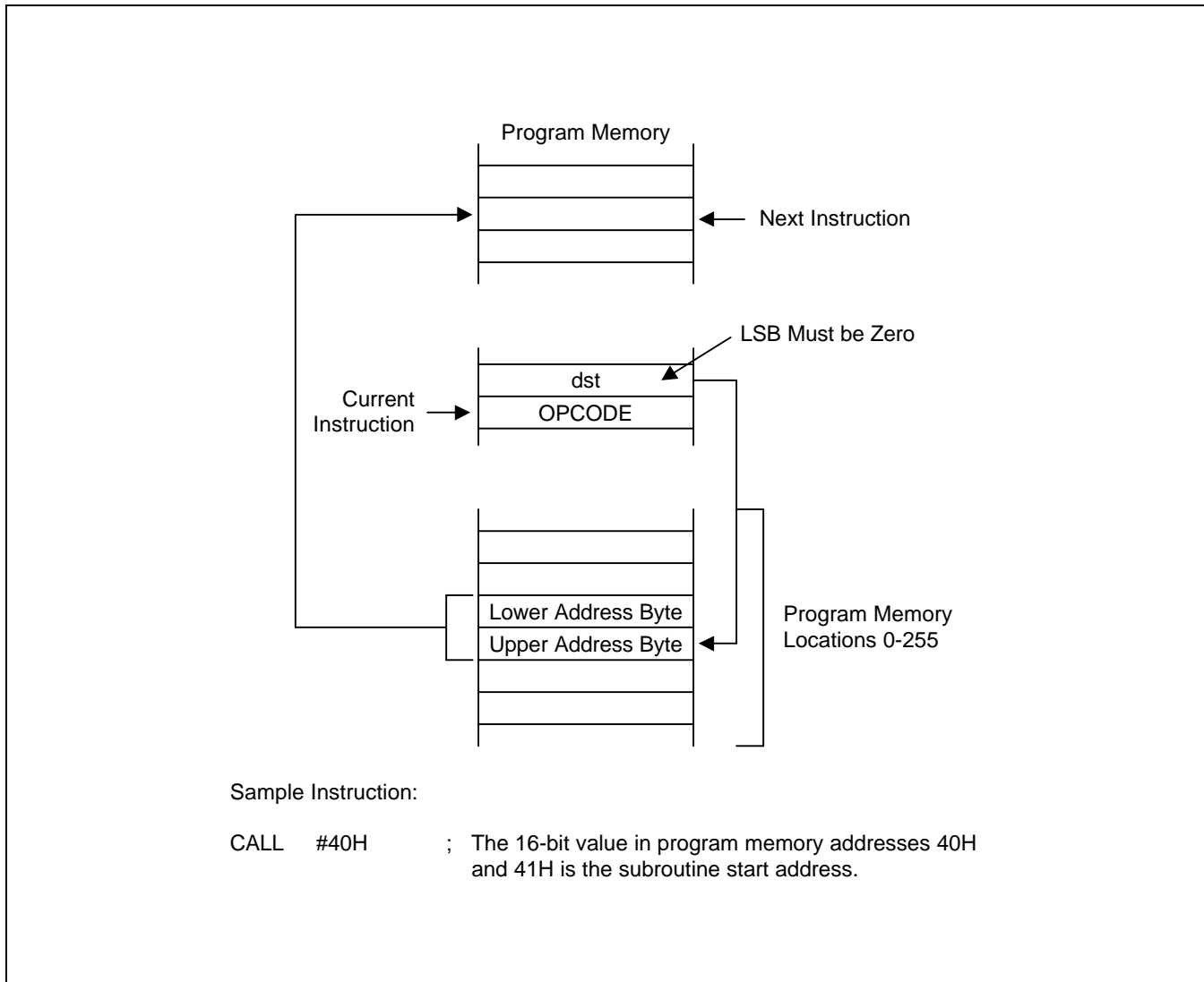
Figure 3-12. Indirect Addressing
