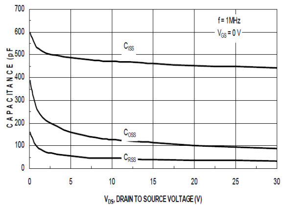
Figure 4. Capacitance Characteristics
