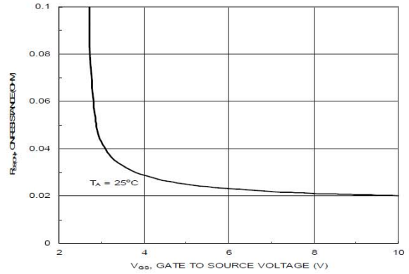
Figure 8. On-Resistance with Gate to Source Voltage
