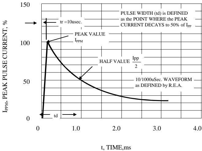
FIG. 3 - PULSE WAVEFORM
