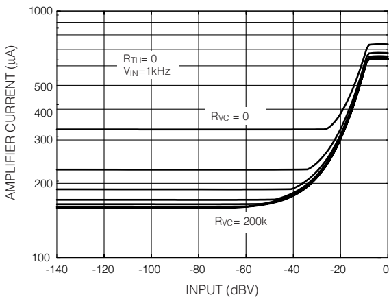
Fig. 8 Amplifier Current vs R_{VC}
