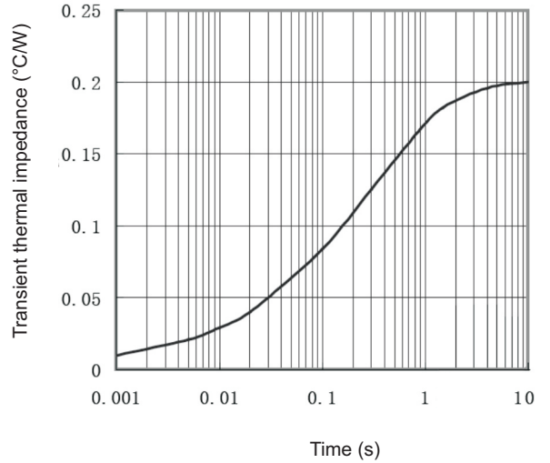
Fig.2 Thermal Impedance (junction to case)
