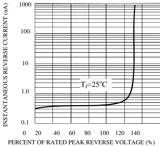
FIG. 3-TYPICAL REVERSE CHARACTERISTICS
