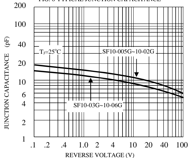
FIG. 6-TYPICAL JUNCTION CAPACITANCE
