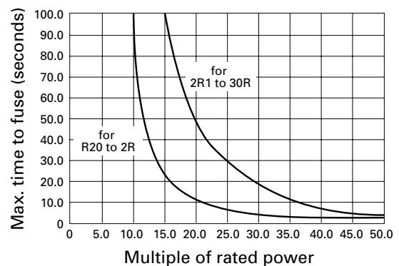
Fusing characteristics for constant current
