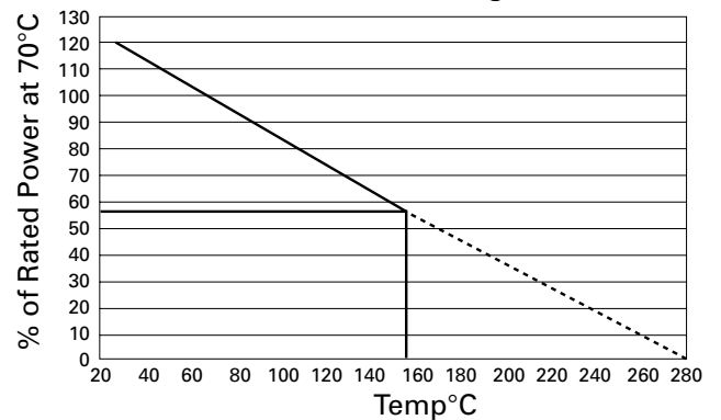
WA84F Series Derating Curve
