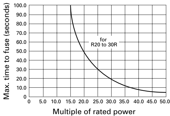
Fusing characteristics for constant voltage
