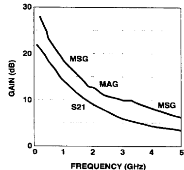
Figure 22. AT-30533 Gains vs. Frequency at V_{CE} = 2.7\text{ V} , I_C = 5\text{ mA} .
