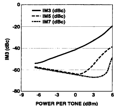
Figure 16. AT-30511 and AT-30533 Intermodulation Products vs. Output Power at V_{CE} = 2.7 V, I_C = 10 mA, 900 MHz with Optimal Tuning.
