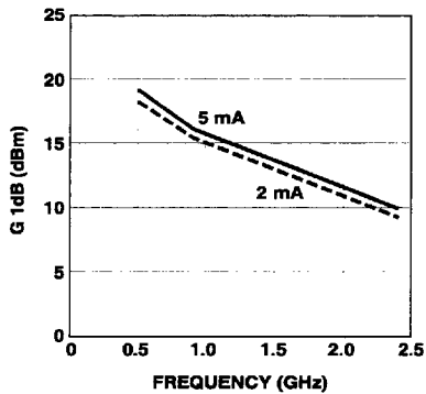
Figure 12. AT-30511 1 dB Compressed Gain vs. Frequency and Current at V_{CE} = 1 V.
