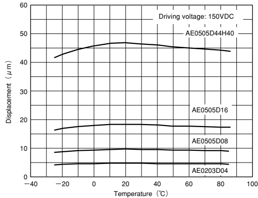
Fig-5 Temperature vs. Displacement
