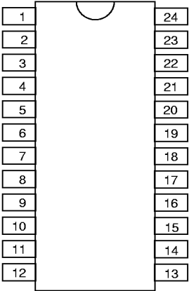
top view 24-pin DIP
