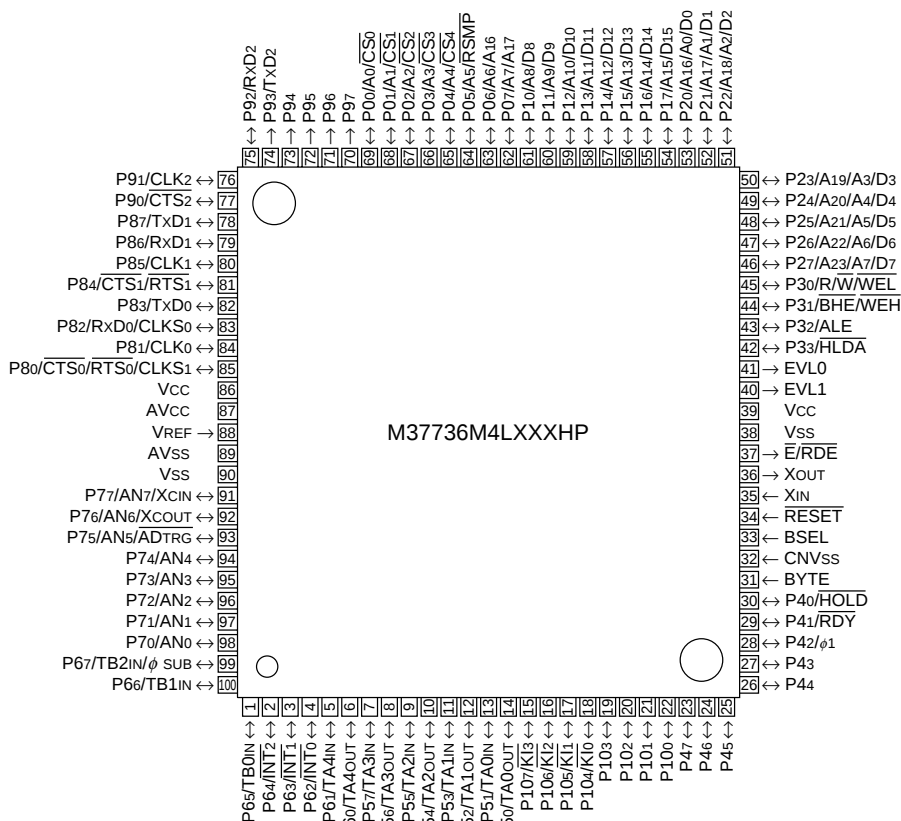
Outline 100P6Q-A
