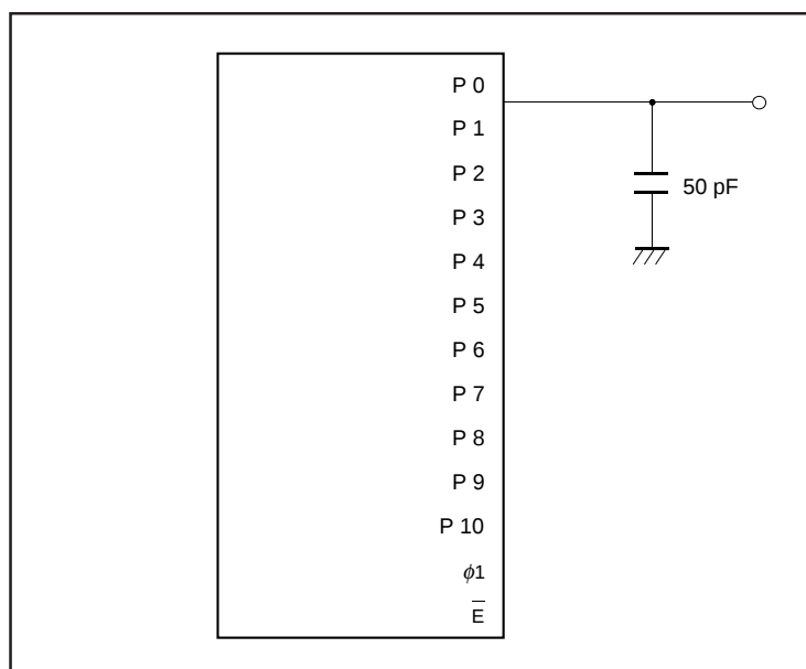
Fig. 7 Measuring circuit for ports P0 - P10 and \phi_1
