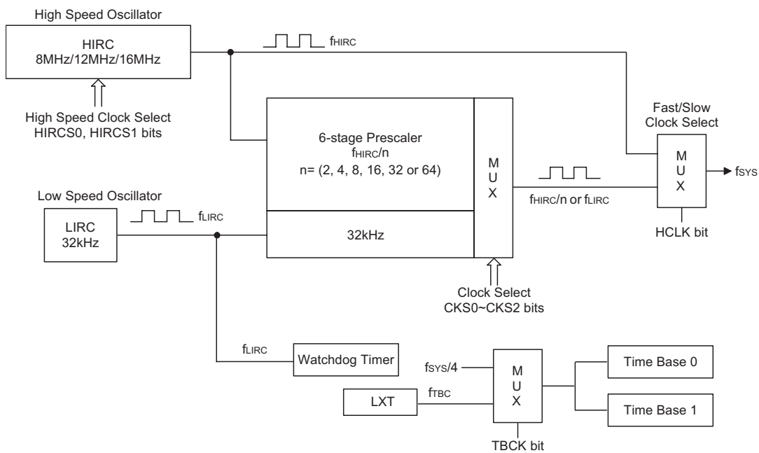
System Clock Configurations – BS85C20-5
