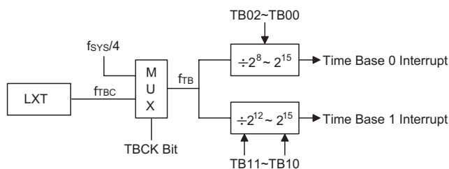
Time Base Structure – BS85C20-5
