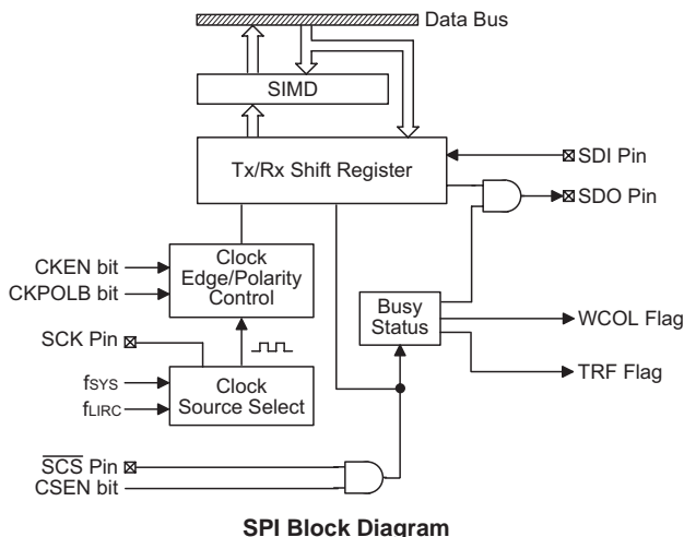
SPI Block Diagram
