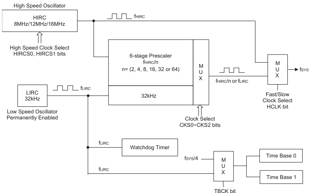
System Clock Configurations – BS85B12-3/BS85C20-3
