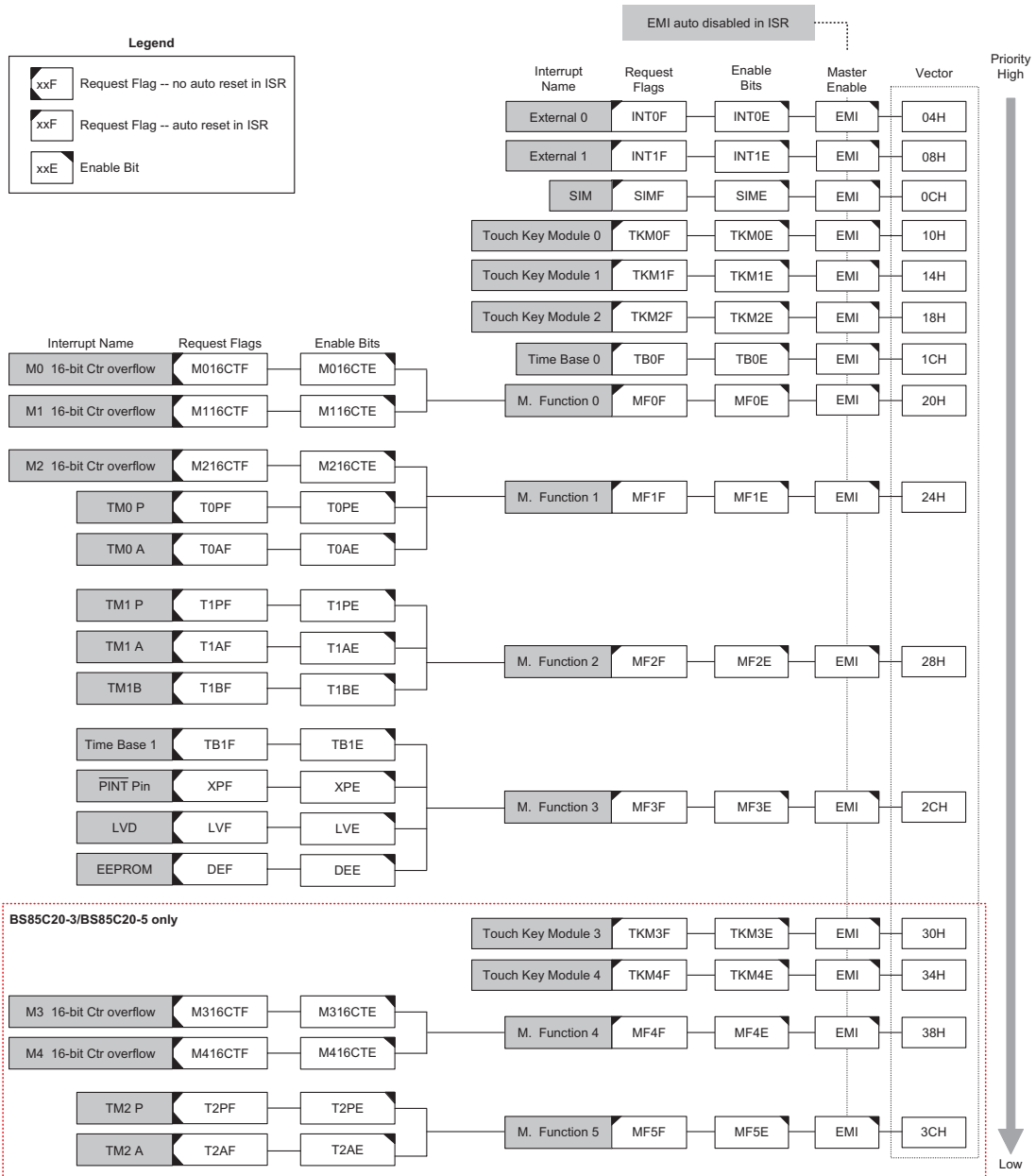
Interrupt Structure
