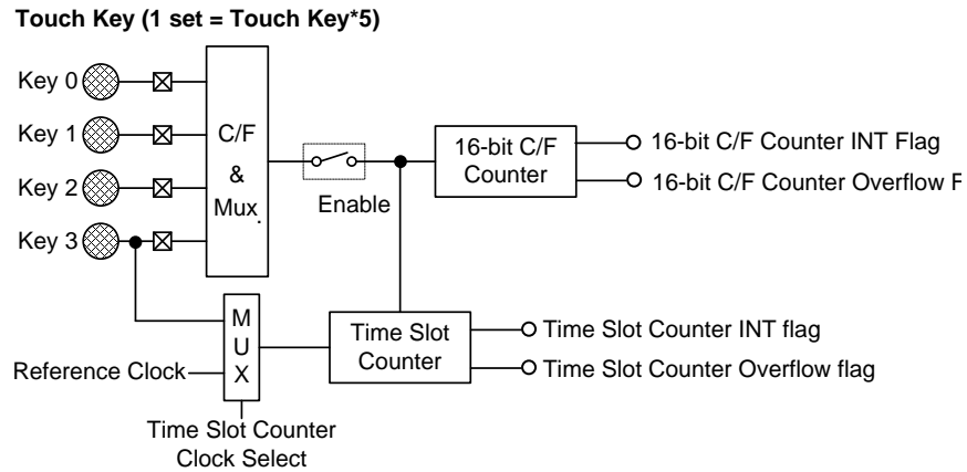
Touch Switch Module Block Diagram
