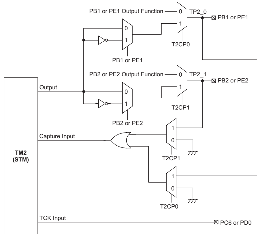
TM2 Function Pin Control Block Diagram – BS85C20-3/BS85C20-5 only
