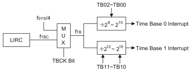
Time Base Structure – BS85B12-3/BS85C20-3
