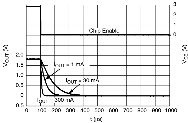
Figure 56. Shutdown, 1.8 V Version D, V_{IN} = 2.8 V
