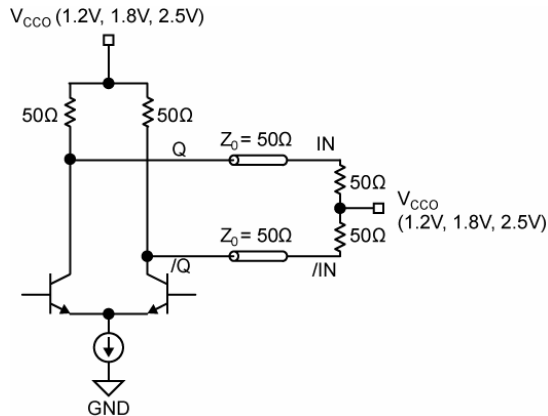
Figure 5a. 1.2V,1.8V, or 2.5V CML DC-Coupled Termination
