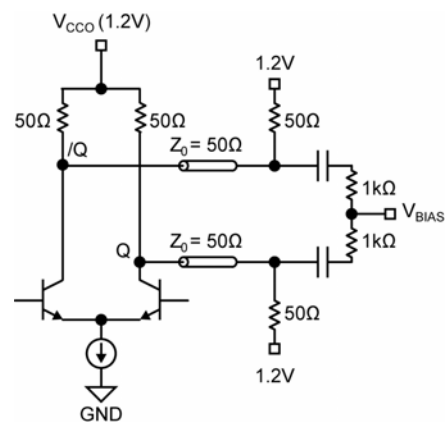
Figure 5d. CML AC-Coupled Termination Vcco 1.2V Only
