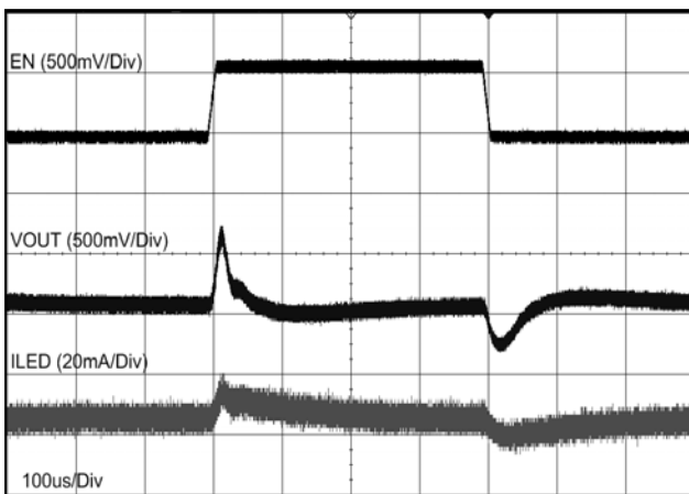
Figure 20. Line Transient Response for 6 LEDs
