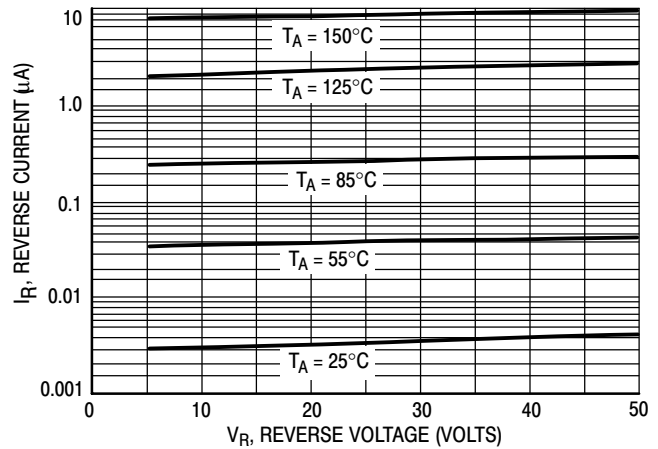
Figure 2. Leakage Current
