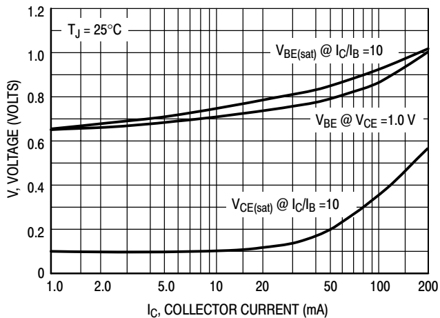
Figure 18. "ON" Voltages
