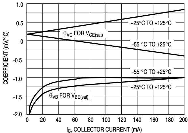
Figure 19. Temperature Coefficients
