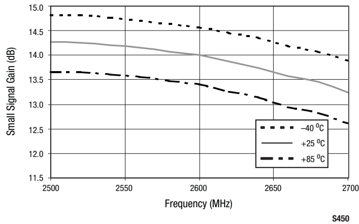
Figure 8. Typical Small Signal Gain From 2500 to 2700 MHz Over Temperature
