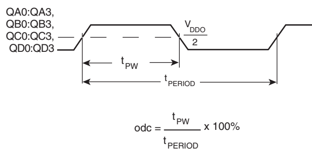
OUTPUT DUTY CYCLE/PULSE WIDTH/PERIOD
